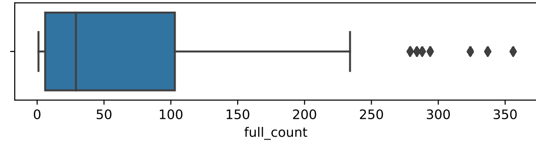
hyper : 90% quantiles
