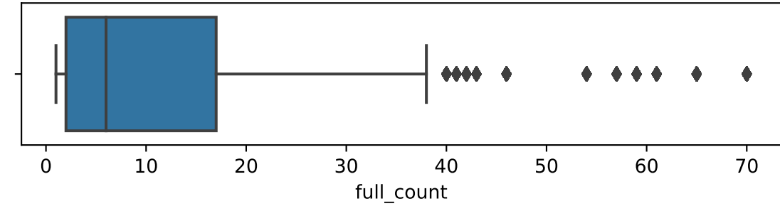
extra : 90% quantiles
