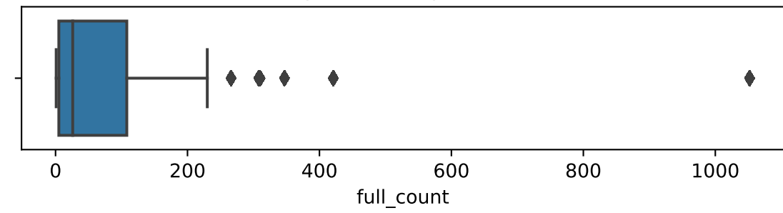
ultra : 90% quantiles
