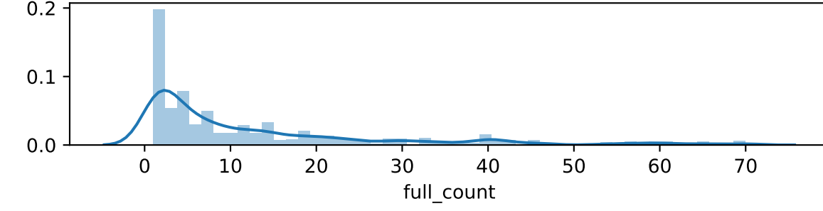
extra : 90% quantiles
