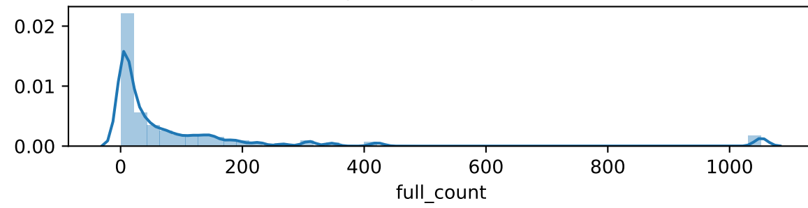
ultra : 90% quantiles
