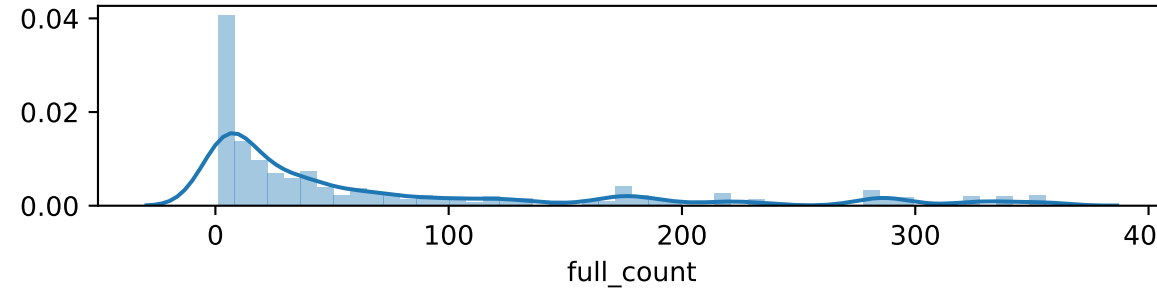
hyper : 90% quantiles
